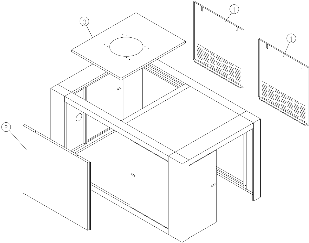
202EDM810 (Ref. Drawing)
